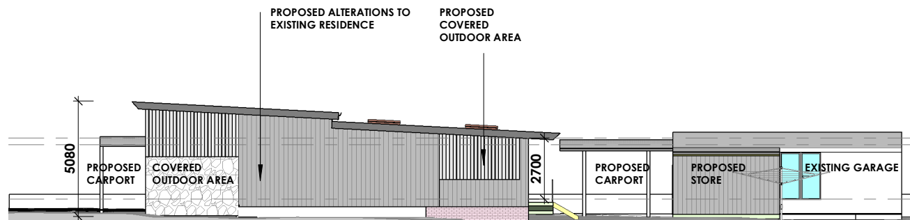
WEST ELEVATION
