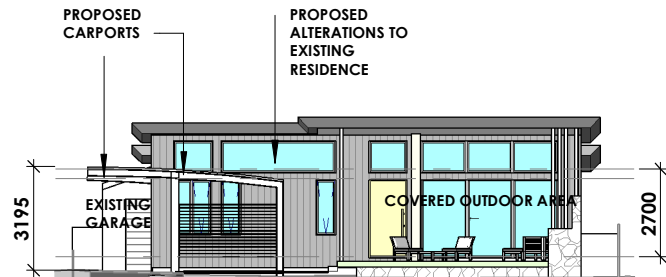
NORTH ELEVATION
