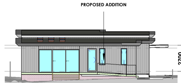
SOUTH ELEVATION
