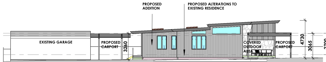
EAST ELEVATION
